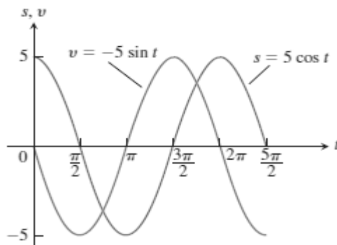
Figure 8.6.1(b): The graphs of the position and velocity of the weight
