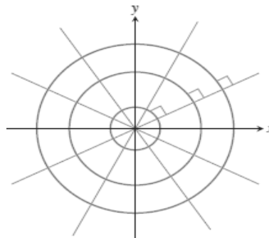
Figure 2: Every straight line through the origin is orthogonal to the family of circles centred at the origin.
