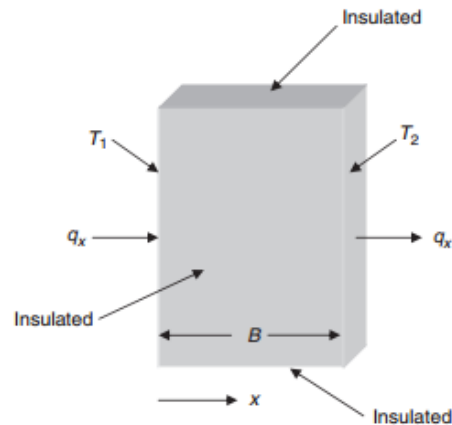
Figure 7.6.2: One-dimensional heat conduction in a solid.
