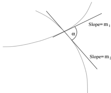
Figure: Oblique ( Or Isogonal)Trajectories
