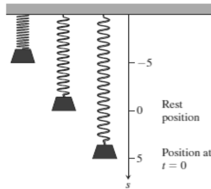
Figure 8.6.1(a): A weight hanging from a vertical spring and then displaced oscillates above and below its rest position
