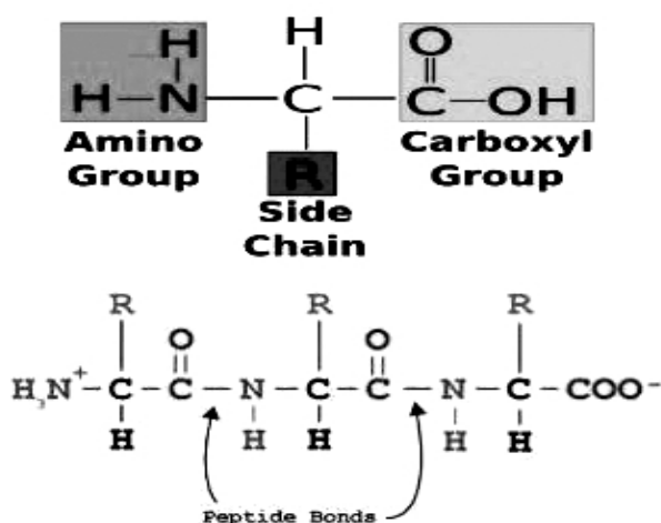
Fig. 4.3 : Primary structure of protein and peptide bond
