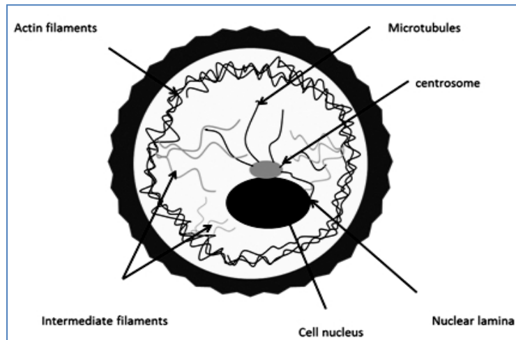
Fig. 2.10 : The cytoskeletal system
