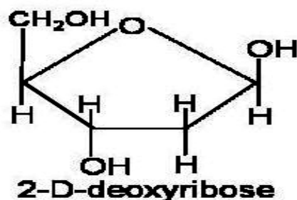
Fig. 3.14 : Deoxy sugar- 2-D- deoxyribose.
