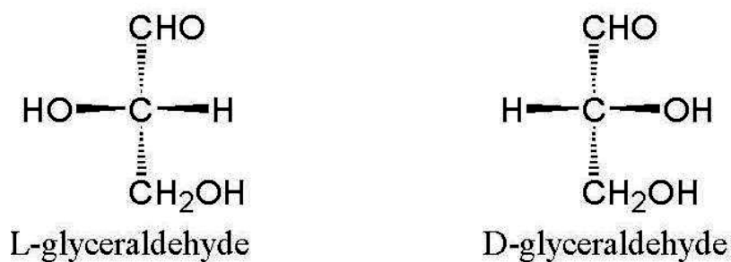
Fig. 3.7 : Glyceraldehyde exists in two isomeric forms that are stereoisomers of each other.
