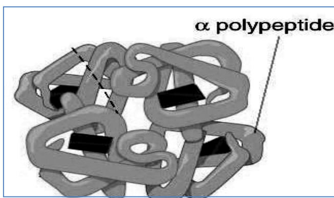
Fig. 4.8 : Quaternary structure of protein.
