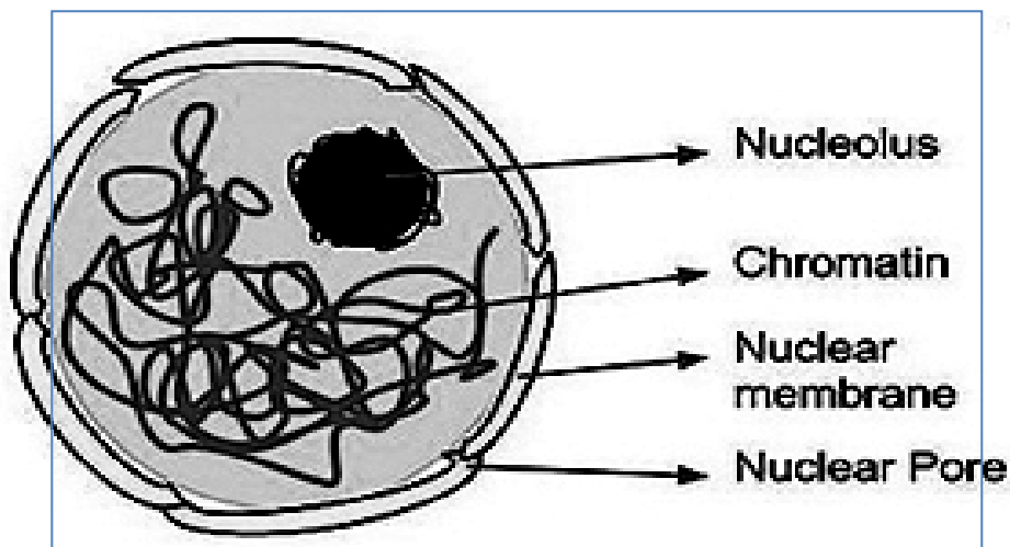
Fig. 2.7 : Structure of nucleus
