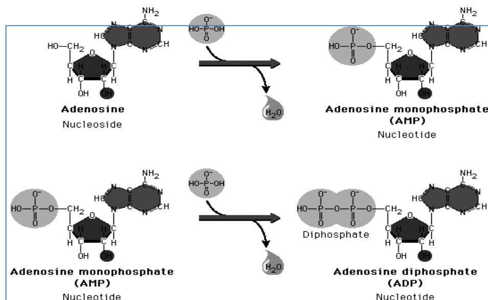
Fig. 6.3 : Structure of phosphate group
