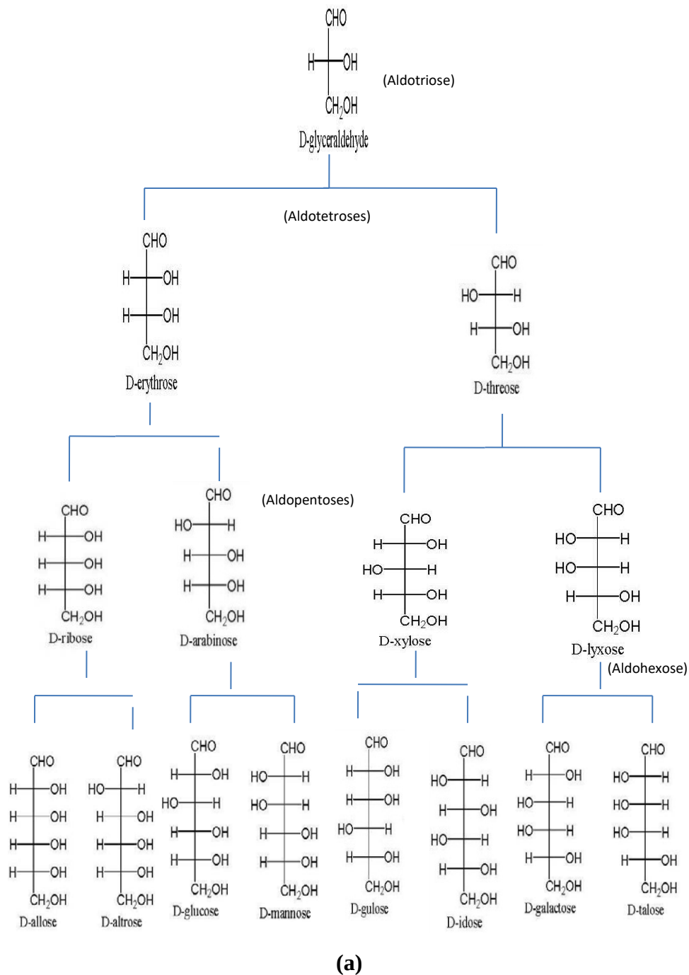
Fig. 3.4 : The monosaccharides: a) glucose an aldohexose having six carbons, b) ribose a ketopentose having five carbons.
