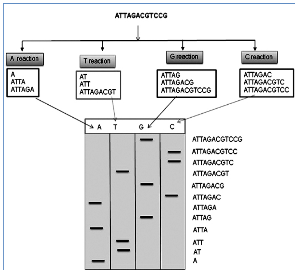
Fig. 6.9 : The Sanger DNA sequencing scheme.
