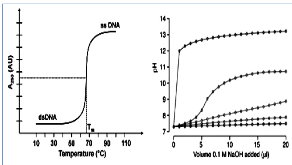
Fig. 6.11 : Effect of tem and pH on denaturation.
