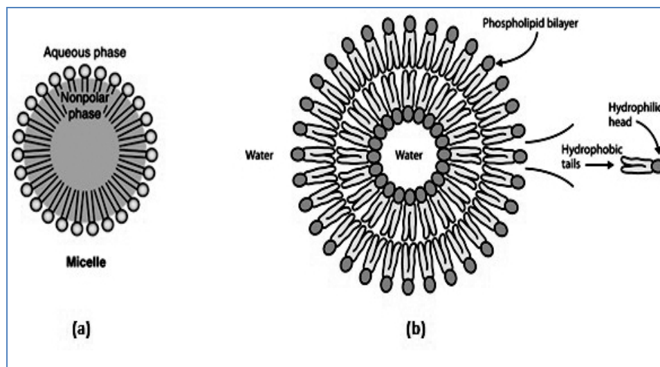
Fig. 5.6 : (a) micelle structure of lipid (b) aggregated structure of glycerolphospholipids and sphingolipids
