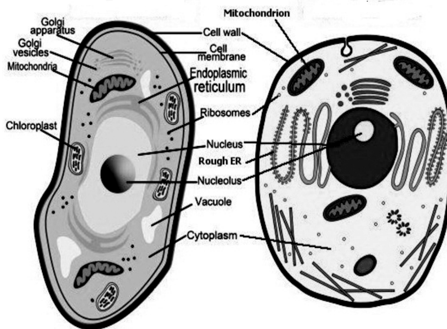
Fig.1.2: Diagram showing: (a) Plant cell (b) Animal cell
