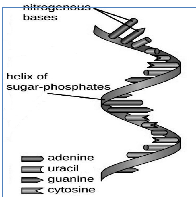
Fig. 6.6 : Structure of single stranded RNA
