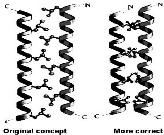
Fig. 4.23 : Structure of Leucine Zipper
