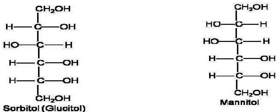
Fig. 3.11 : Sugar alcohol, sarbitol and mannitol.
