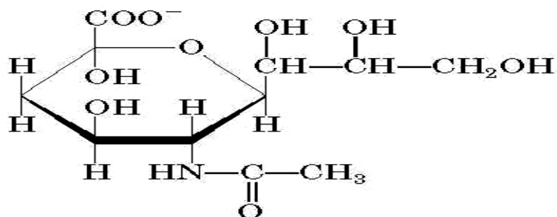
N -Acetylneuraminic acid (a sialic acid) (Neu5Ac)
