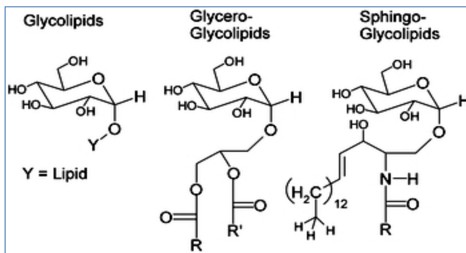
Fig. 5.3 : Structure of glycolipids
