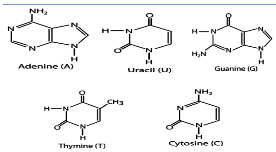
Fig. 6.1 : Structure of nitrogenous bases.
