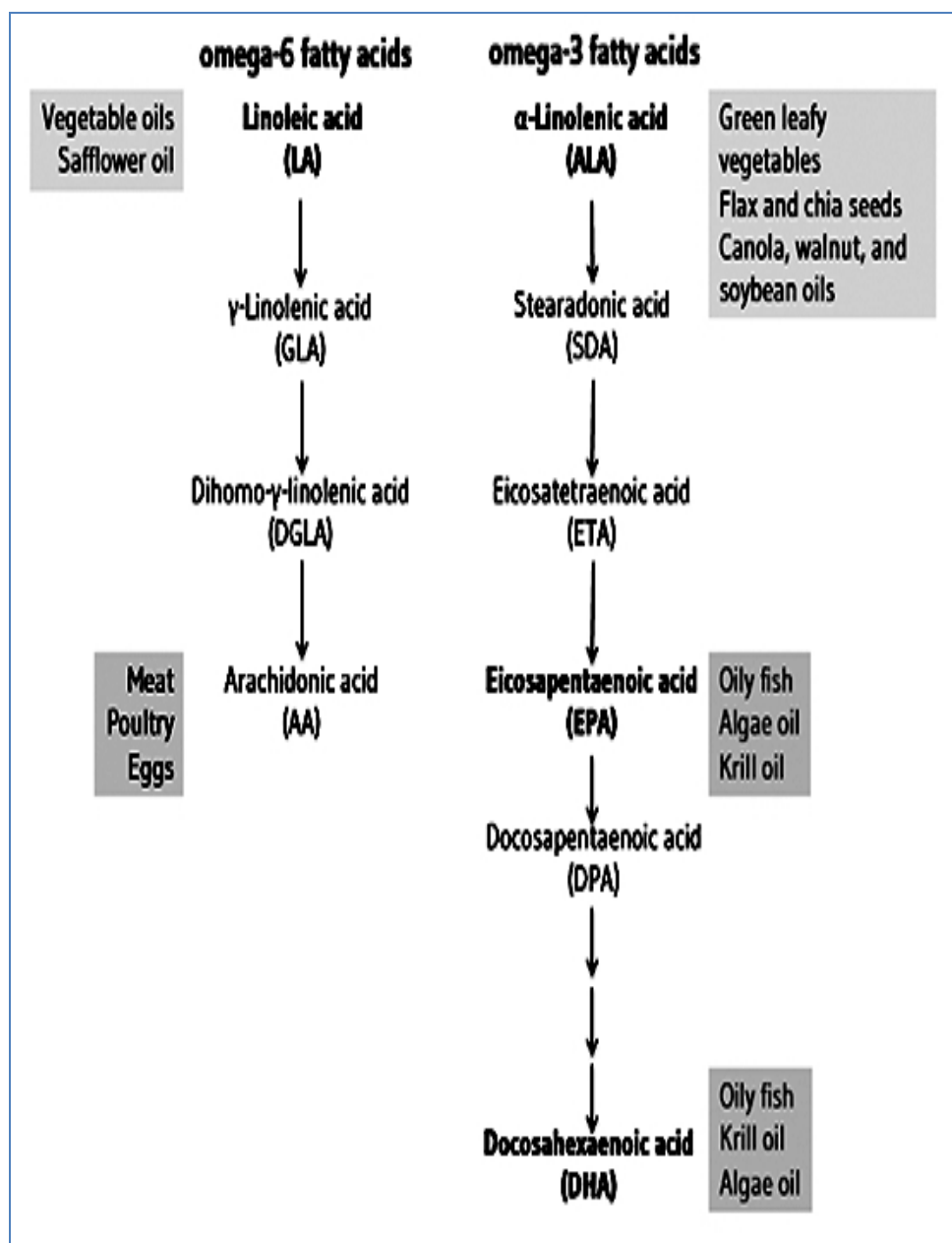
Fig. 5.2 : Classes of essential fatty acids
