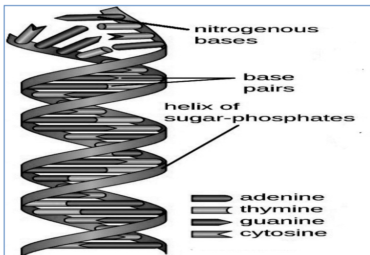
Fig.6.4 : Structure of double stranded DNA
