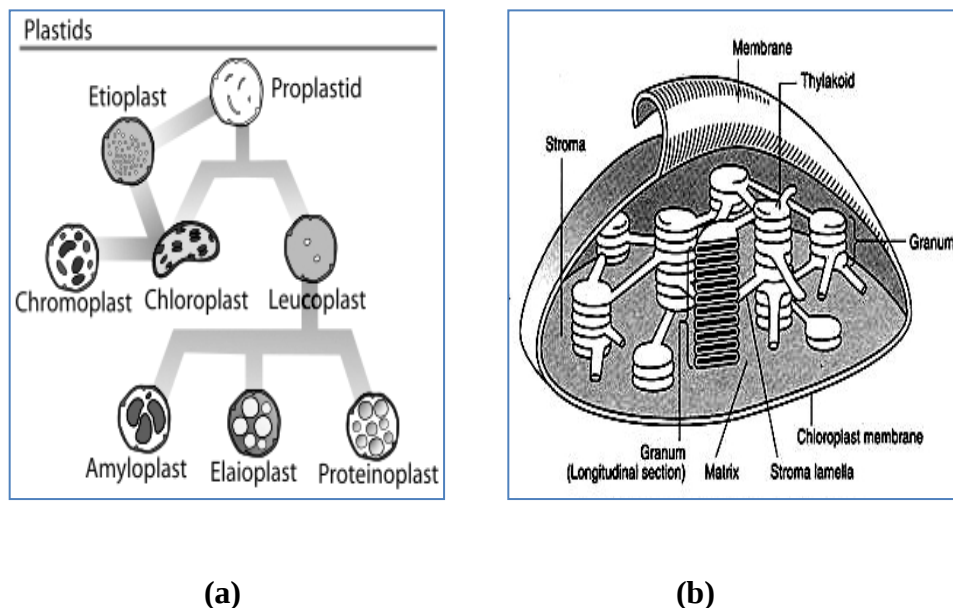
Fig. 2.6 : a) Structure of different types of plastids, b) three dimensional structure of chloroplast.
