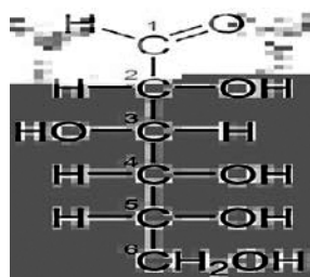
Fig. 3.2 : Structure of Glucose
