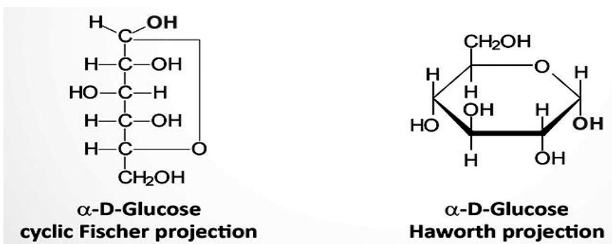
Fig. 3.3 : Fisher and Haworth projection in monosaccharides
