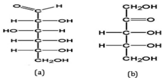
Fig. 3.4 : The monosaccharides: a) glucose an aldohexose having six carbons, b) ribose a ketopentose having five carbons.
