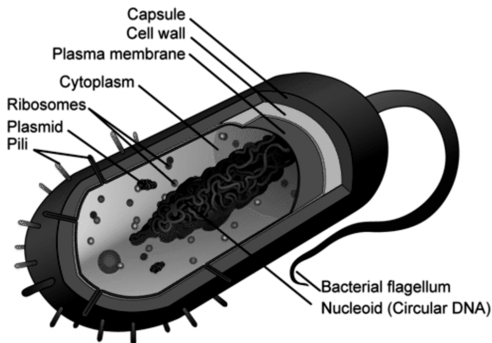
Fig. 1.1 : Diagram of prokaryotic cell
