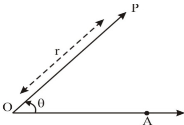
Fig. polar coordinate
