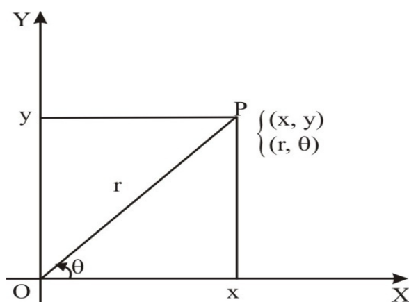
Fig. : Polar and Cartesian Coordinates.
