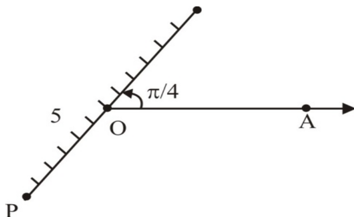
Fig.1 : P's polar coordinates are \left(-5 - \frac{\pi}{4}\right)
