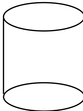
Fig. 5.4 (Right Circular Cylinder)
