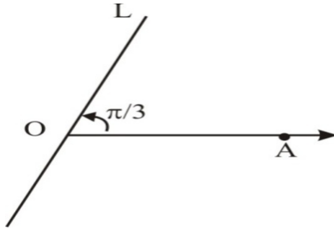
Fig.2 : The line L is given by \theta = \pi/3 .
