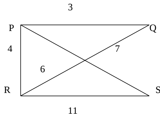
Fig 10.2 Weighted Graph
