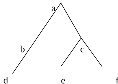
Fig 10.7 Tree
