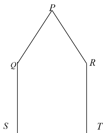
Fig. 10.3 Labeled Graph
