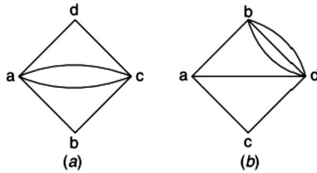
Fig.5 Multigraph
