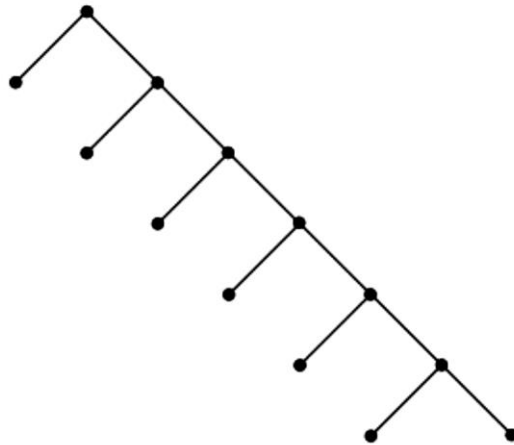
Fig. 8 Binary tree of maximum height with 13 vertices
