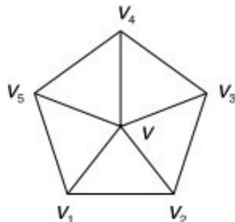
Fig.16 Wheel graph ( W_6 )
