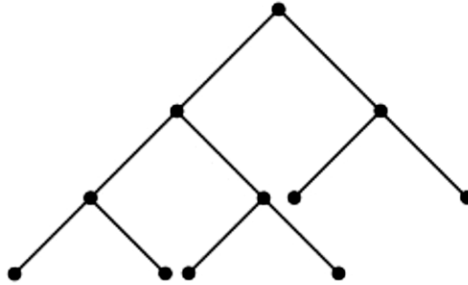
Fig. 5 Binary tree
