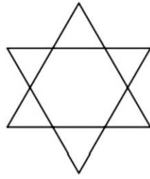
(b) Complement \bar{G} of G
