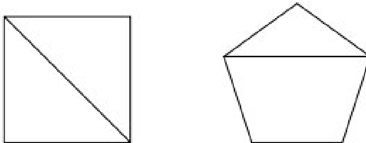
Fig. 6 Simple graphs
