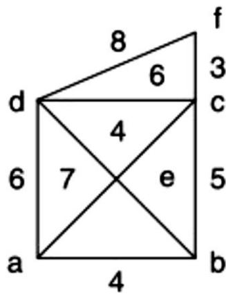
Fig.9 Weighted graph
