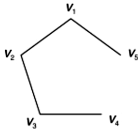
Fig.15 Path graph of order 5 ( P_5 )
