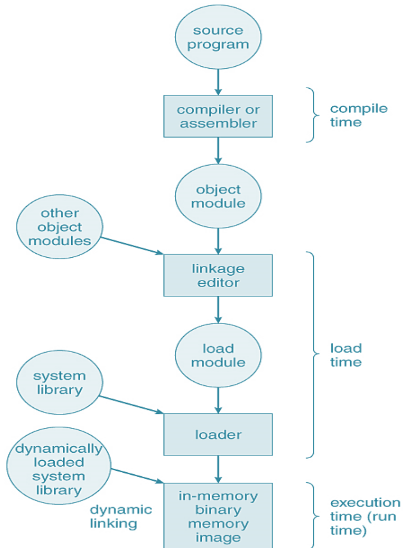
Figure 6.3 Multistep processing of a user program
