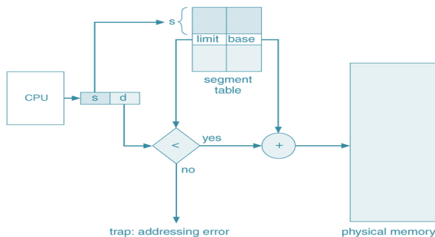
Figure 6.17 - Segmentation hardware
