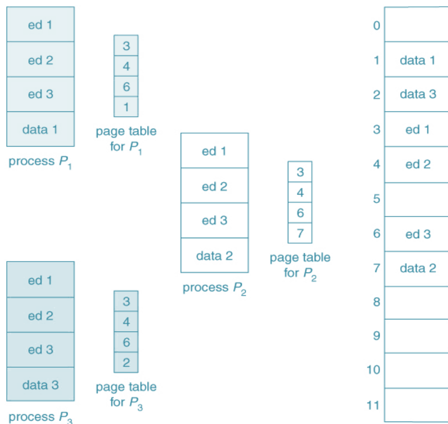
Figure 6.14 : Sharing of code in a paging environment
