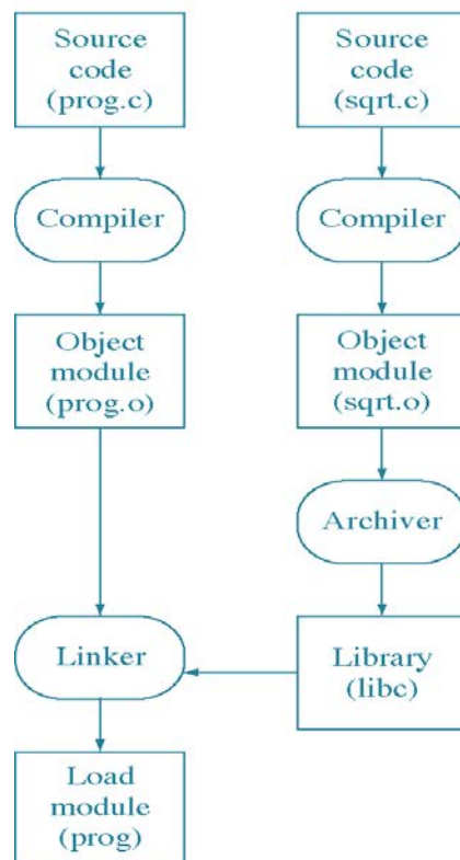
Figure 6.4 Creating a load module
