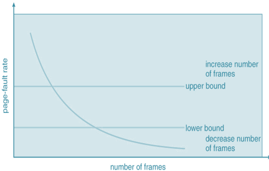
Figure 6.30 : Page-fault frequency
