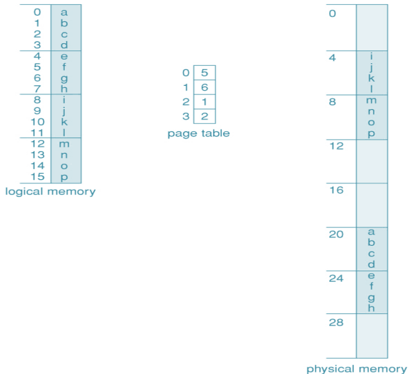
Figure 6.10 Paging example for a 32-byte memory with 4-byte pages
