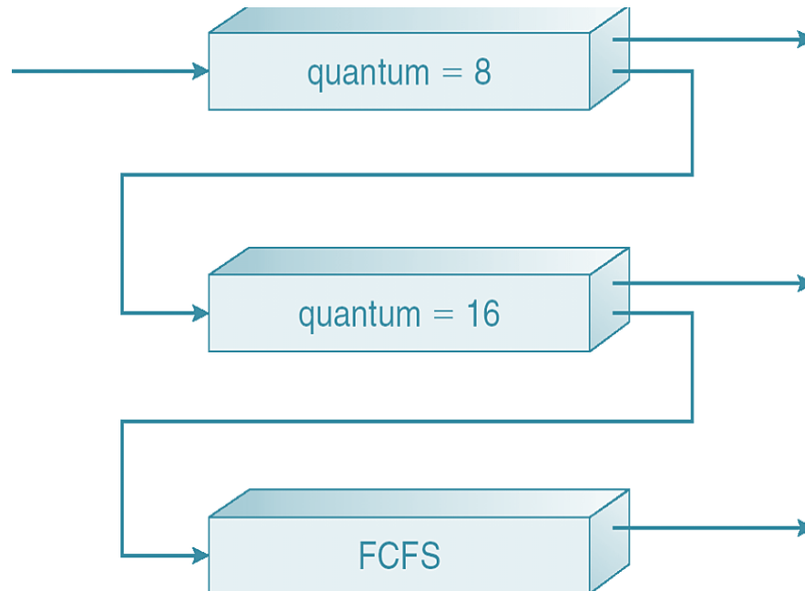
Figure - 3.4 Multilevel Feedback Queue Scheduling
