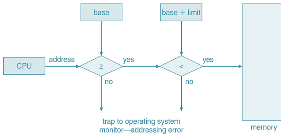
Figure 6.2 : Hardware address protection with base and limit registers
