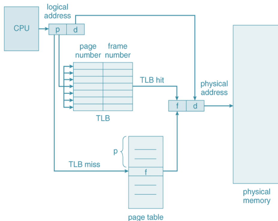
Figure 6.12 : Paging hardware with TLB
