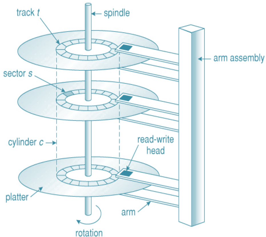
Figure 7.1 : Moving-head disk mechanism
