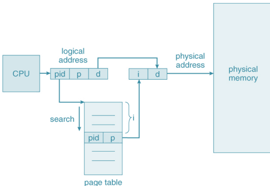
Figure 6.16 : Inverted page table
