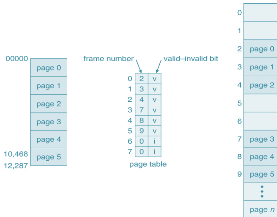
Figure 6.13 : Valid (v) or invalid (i) bit in page table
