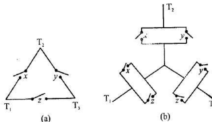
Delta-to-wye transformation
