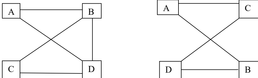
Undirected Graph
