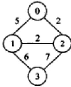
Weighted Graph
