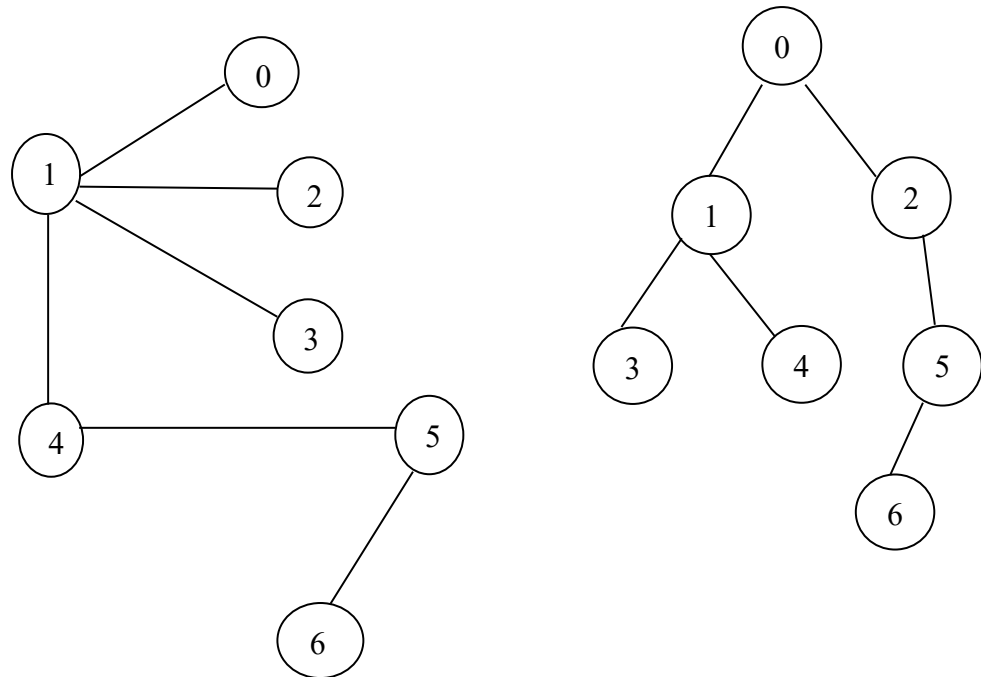
Spanning Trees
