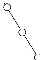
Right Skew
