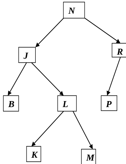
Step 7
