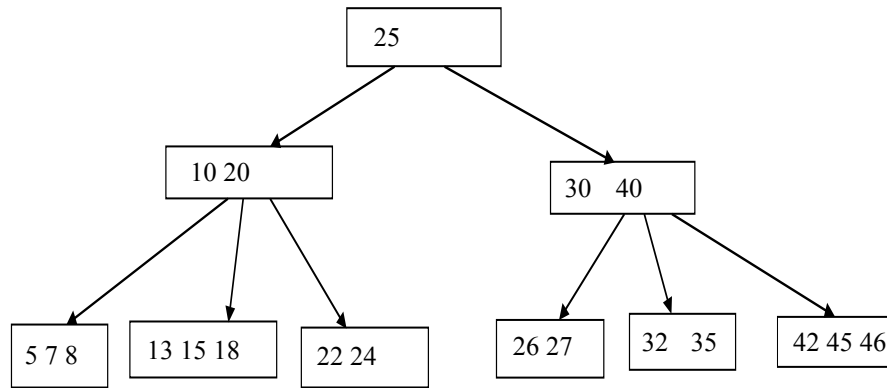
Step 1
