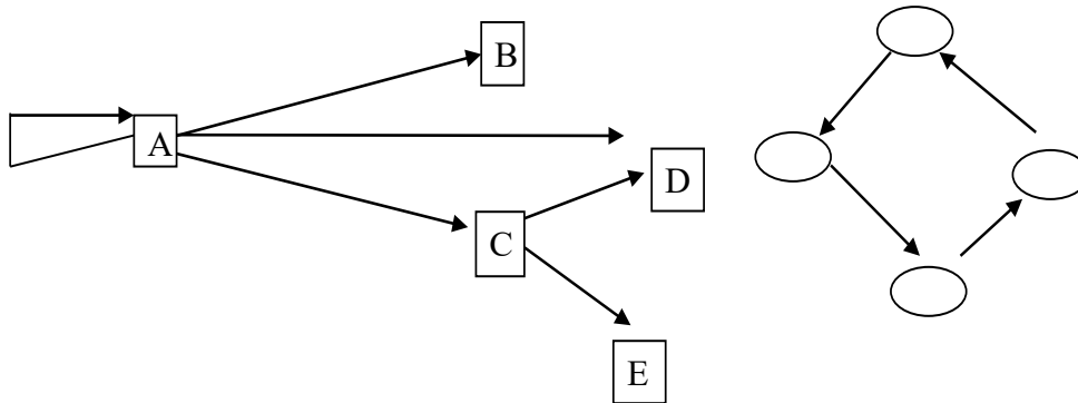
Directed Graphs
