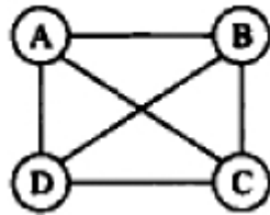
Connected Graph
