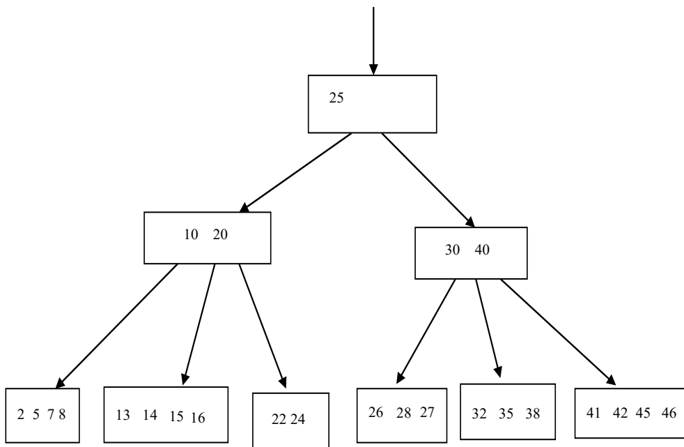
B-Tree of order 5 with level 3
