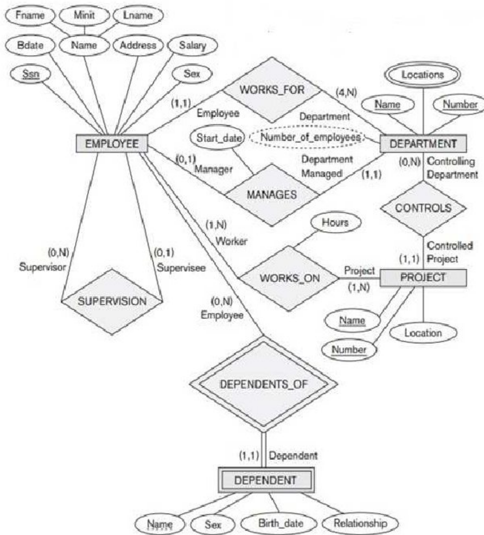
Figure 3.9- Refined ER Diagram of the company database [1] .
