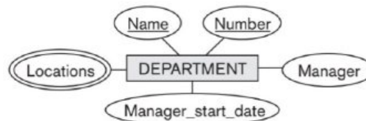
Figure 3.4- A Department entity type [1] .
