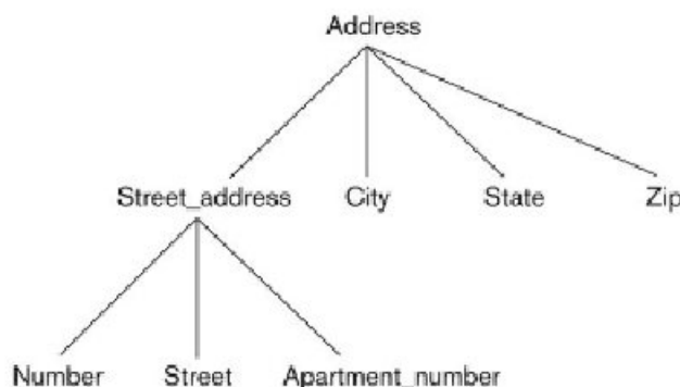
Figure 3.2- Address is a composite attribute of employee entity set iii .
