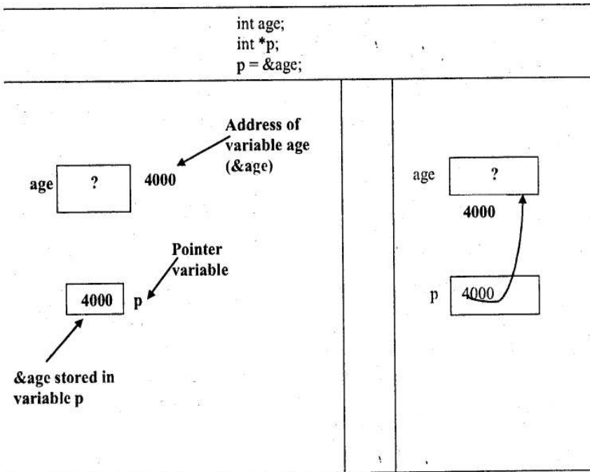
Figure 1.1: Memory and logical representation of pointer variable
