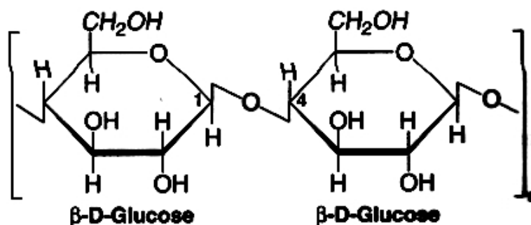
Fig. 6.12: Structure of cellulose
