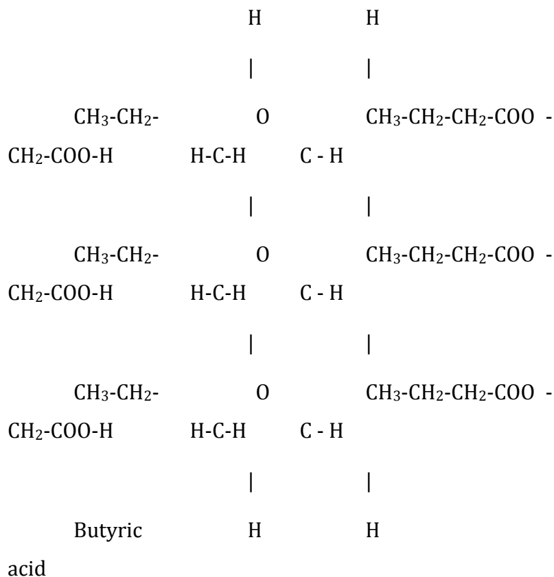
Fig. 7.5: Chemical formulae of Tributyrin
