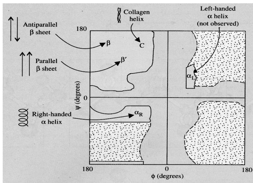
Fig.5.2: Ramachandran Plot
