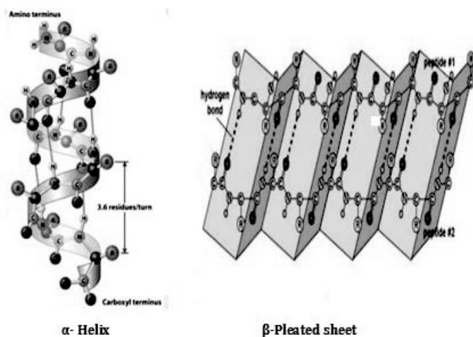
Fig. 5.1: Secondary structure of protein
