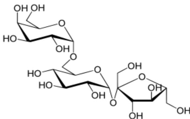
Fig.6.8: Chemical structure of trisaccharides – raffinose
