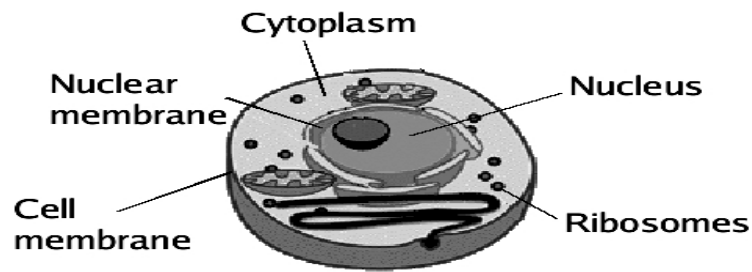
Fig. 3.6: Structure of ribosomes in cell
