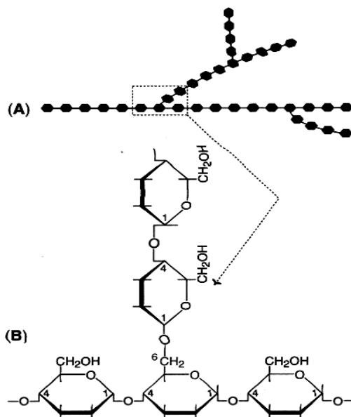
Fig. 6.11: Structure of Glycogen (A) General structure (B) Enlarged at a branch point
