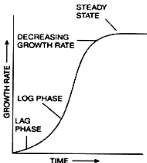
Fig. 17.1. Sigmoid curve.
