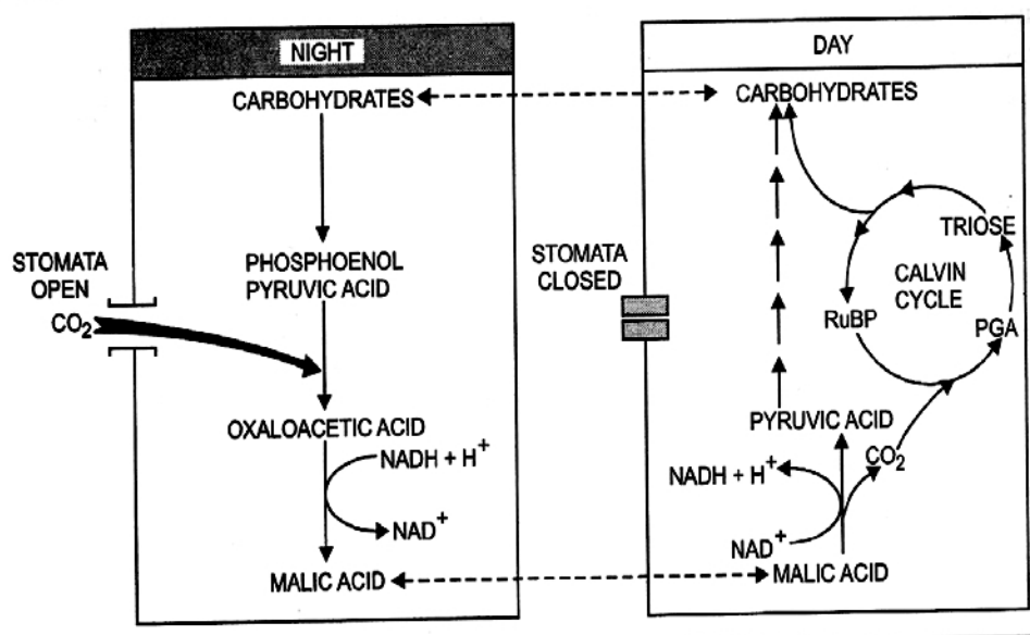
Fig 6.7 CAM Cycle
