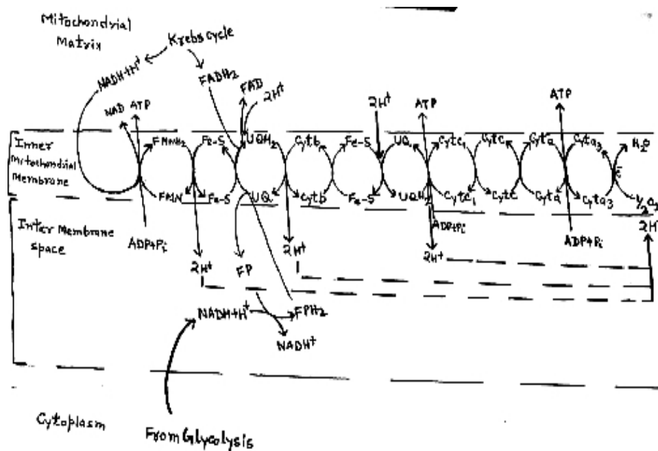
Fig 8.3 ETS cycle
