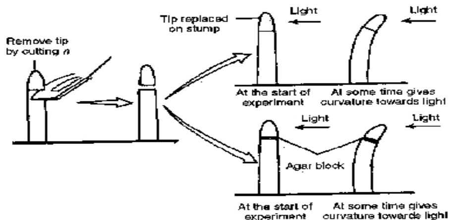
Fig 7.3 Boysen-Jensen experiment.
