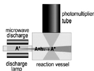
Fig.6.19 Resonance fluorescence
