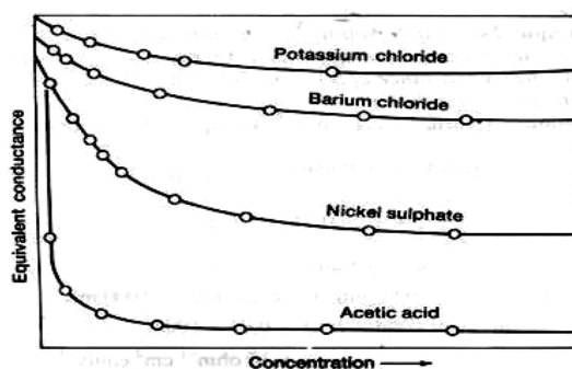
Fig.5.2 Conductance curve
