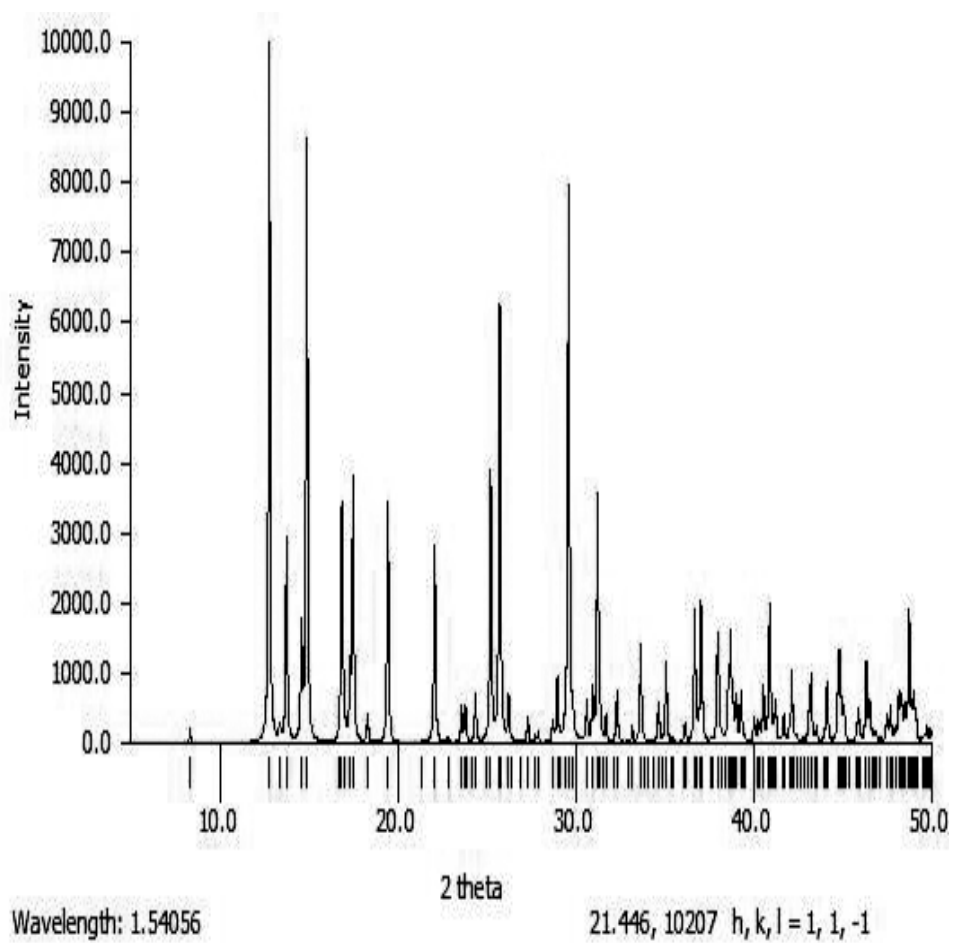
Figure 8: Simulated PXRD of compound 1: generated by Mercury software
