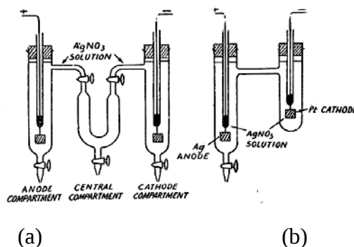
Fig. 5.7 Hirtoff cell
