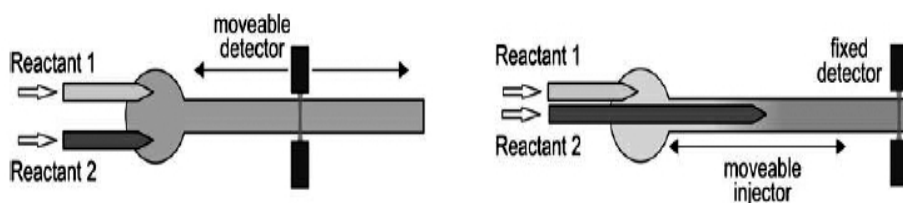
Fig. 6.15 Continuous flow technique
