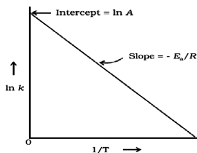
Fig. 6.24 : A plot between \ln k and 1/T
