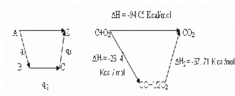
Fig.4.11 Thermal effect depend on initial and final state
