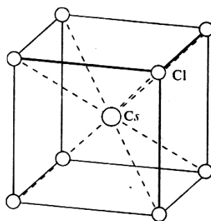
Figure: Cesium chloride crystal lattice
