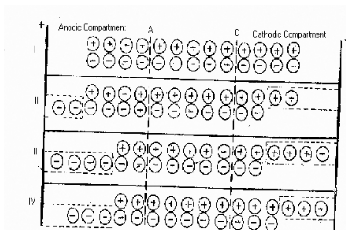
Fig. 5.5: Anodic and Cathodic compartments showing speeds of migration of ions during electrolysis
