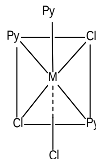
mer-trichlorotripyridinerhodium(III)
