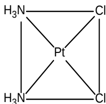
cis-dichlorodiammineplatinum(II)
