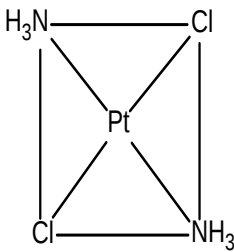
trans-dichlorodiammineplatinum(II)
