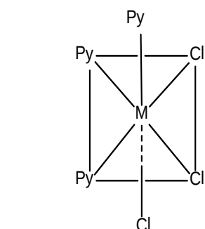
fac-trichlorotripyridinerhodium(III)
