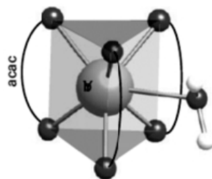
1. Complex [\text{Yb}(\text{acac})_3(\text{OH}_2)]
