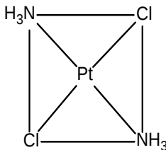
trans-dichlorodiammineplatinum(II)
