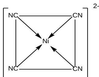
dsp^2 -hybridized square planar complex
