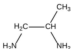
1,2-diaminopropane
