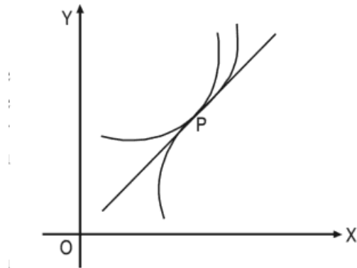
Figure 10: double cusp with change of species
