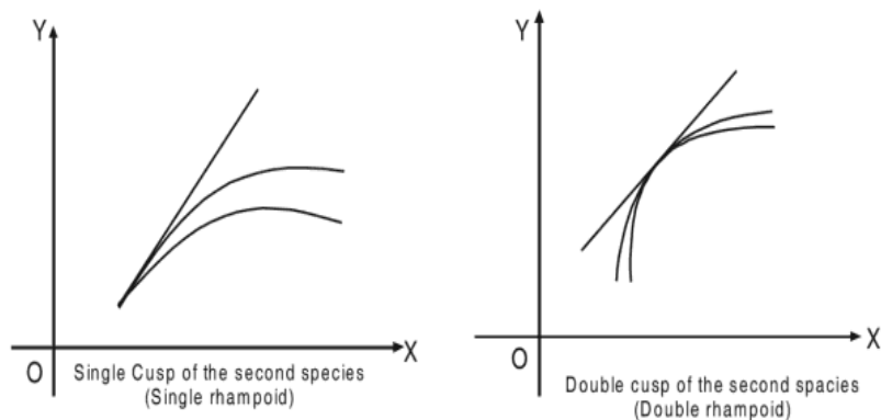
Figure 9: Second species of cusp
